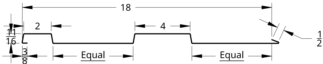
Unequal battens, 2" minimum, 6" maximum
