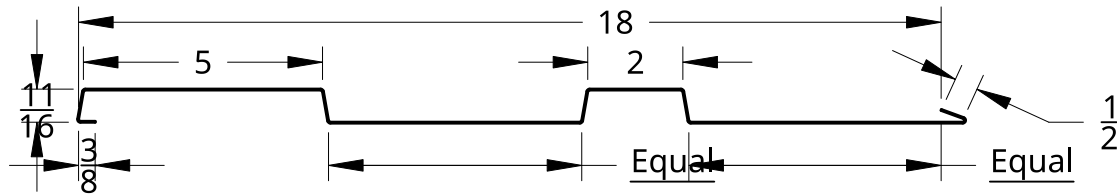
Equal battens, 2" minimum, 6" maximum
